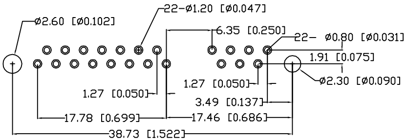
RECOMMENDED P.C. BOARD LAYOUT COMPONENT SIDE SHOWN
