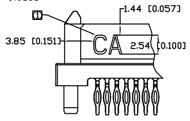
VIEW B
